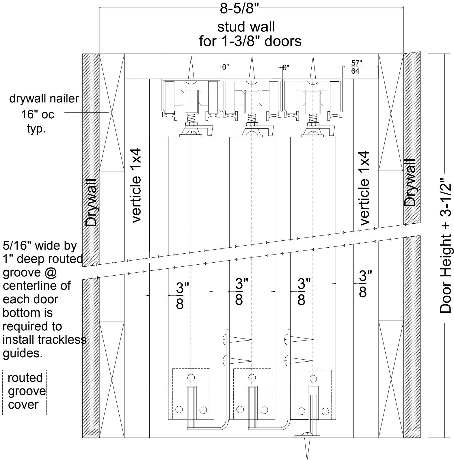
3 Door multipass frame section for 1-3/8" doors
