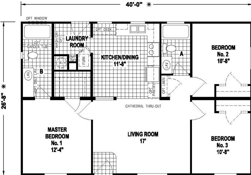
9200CT/4028 (1,066 SQ. FT.) 3BEDROOM - 2BATHS - CATHEDRAL THRU-OUT
