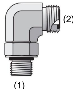
STRAIGHT THREAD ELBOW ORB / ORFS (C5OLO)
