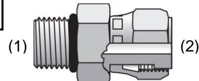
STRAIGHT THREAD SWIVEL CONNECTOR ORB / ORFS (F65OL)
