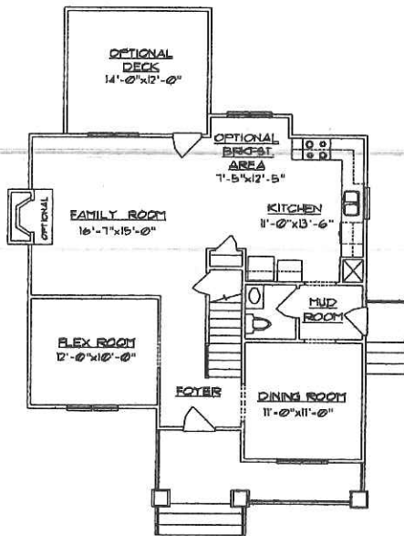
FIRST FLOOR PLAN 923 SQ. FT. (HEATED)
