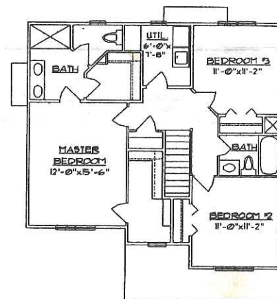
SECOND FLOOR PLAN 306 SQ. FT. (HEATED)
