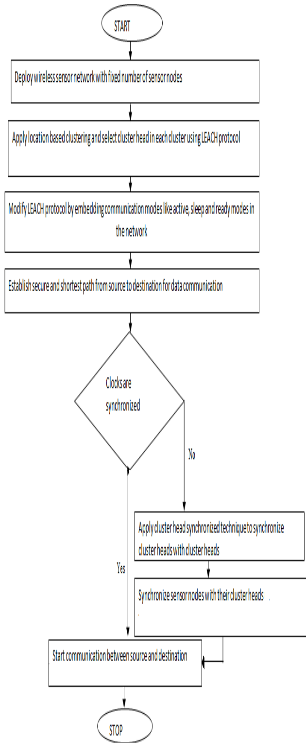
Fig.1: Proposed Flowchart
