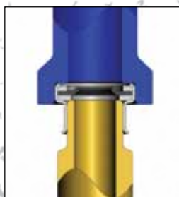
Seal Installation Detail
