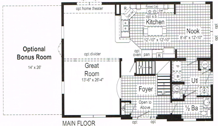
MAIN FLOOR
