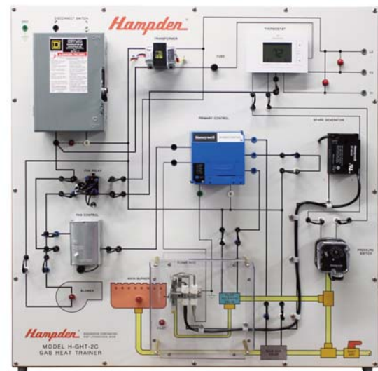
Model H-GHT-2C Gas Heat Trainer
