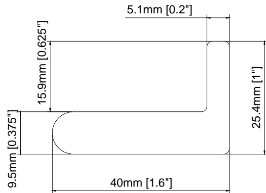
1.6" Sill plate with 5/8" light block
