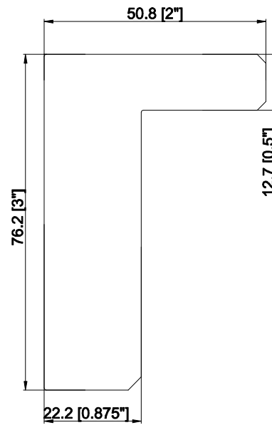
Mission sill Frame
