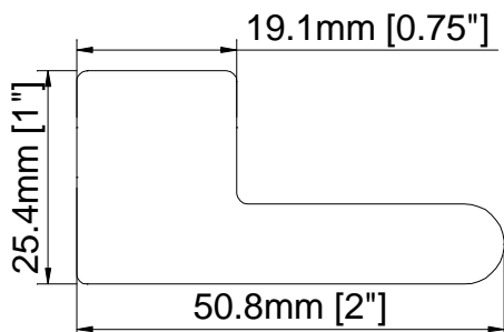
2" Sill Plate with 5/8" Light Block (L/Z)
