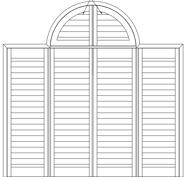
Standard unit with horizontal arch center
