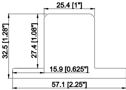
1" Chamfer T Post W/ 1/4" Light Block (Deco)
