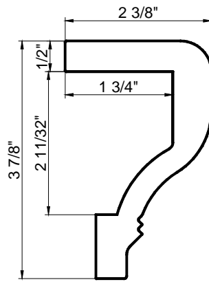
Curved Designer Sill Cap (D/HS)
