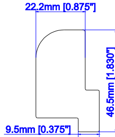
Tilt Out Z Frame
