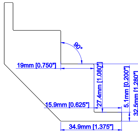
Corner Post W/ 1/4" Light Block (Deco)
