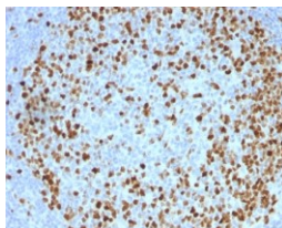
FFPE human tonsil stained with anti-TOP IIA using DAB
