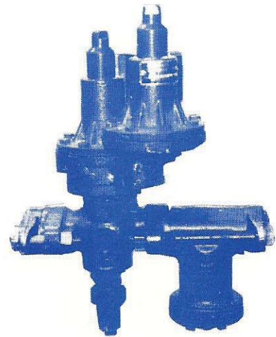
3/4" AND 1" A4A (2-BOLT FLANGES) W/2 MODULES AND STRAINER
