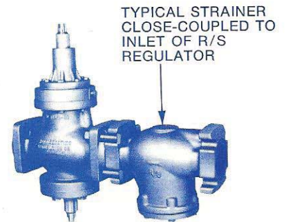
1-1/4" THRU 4" A4A W/STRAINER (4-BOLT FLANGES)
