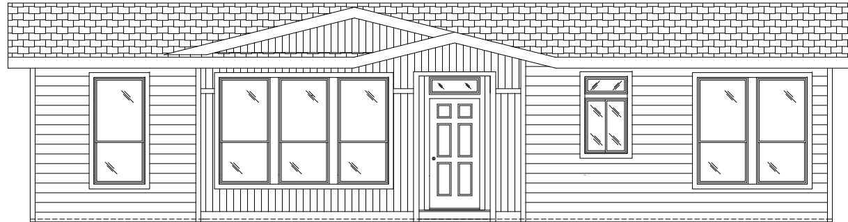
FRONT SIDEWALL W/NOMINAL 24'-0" EYEBROW DORMER
