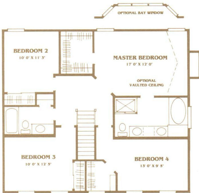
SECOND FLOOR
