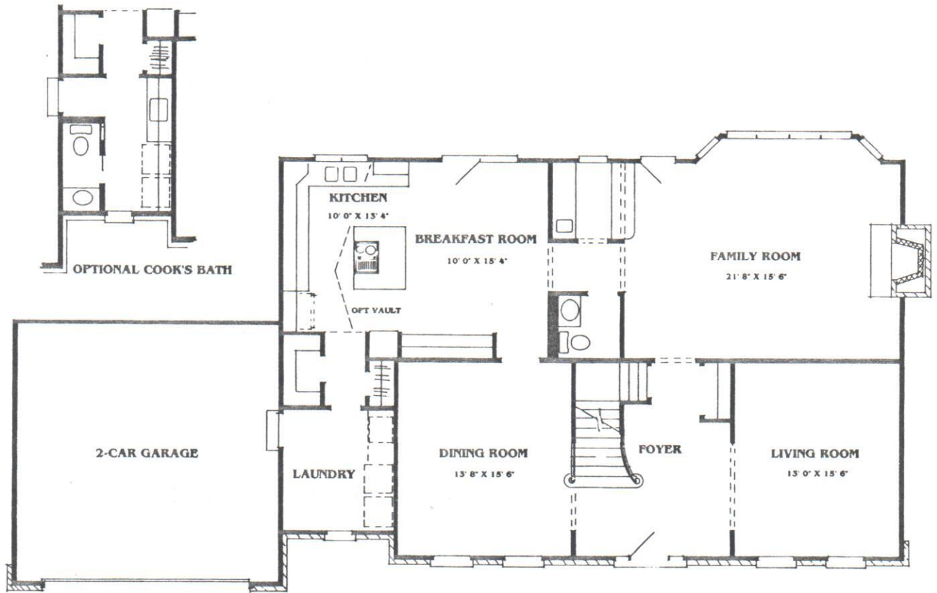
FIRST FLOOR
