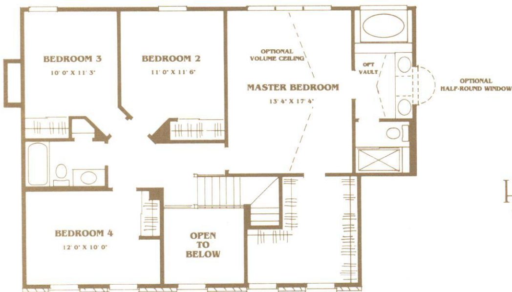
SECOND FLOOR
