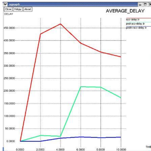
Figure.3 Simulation results for PEDM-ACO
