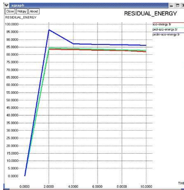
Figure.5 Comparison of Residual Energy for the heuristic techniques of network
