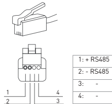
Data Cable: RJ9
