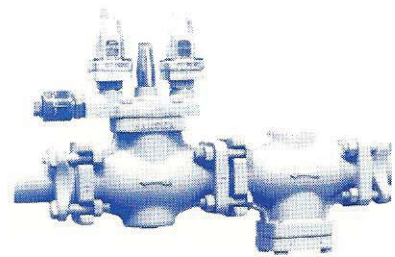
1-1/4" THRU 4" SQUARE FLANGED HA4AD WITH AND WITHOUT STRAINER
