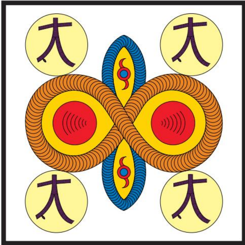
(Symbol - Overpopulation)
