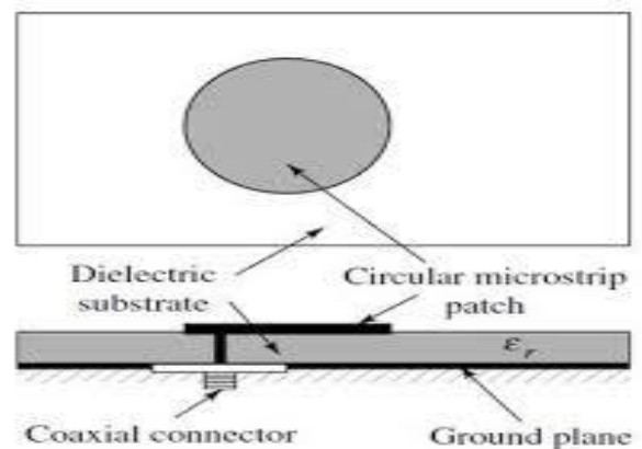
Fig.1: Antenna substrate
