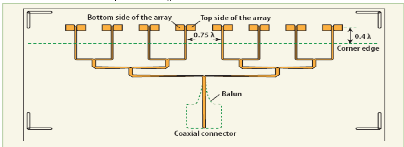
1. This layout represents the printed patch array antenna with feed network and balun.
