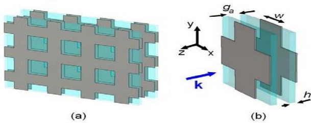
Fig.2. (a) Schematic view of MENZ metamaterial based on the fishnet structure (b) metamaterial unit cell
