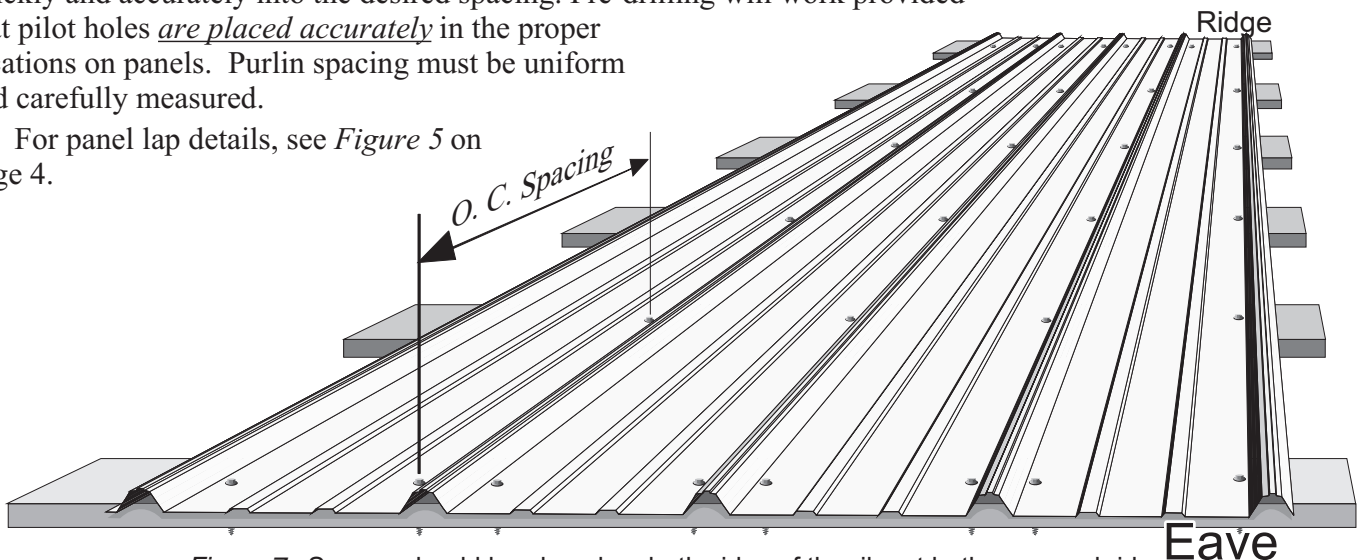
Figure 7 Screws should be placed on both sides of the ribs at both eave and ridge.
