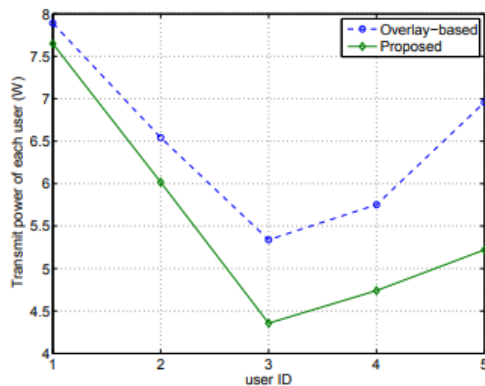
Figure 7: The transmit intensity of Sus versus client ID with various asset assignment systems
