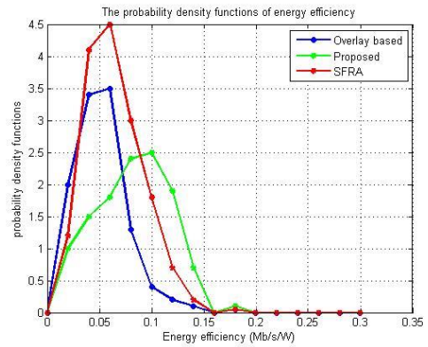
Figure : The likelihood thickness elements of vitality productivity with various asset portion methodologies.
