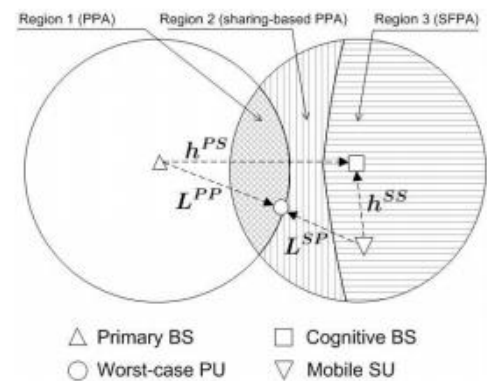
Figure 2.1: A CR framework existing together with an essential framework (uplink situation for the CR framework). Three locales are featured for the CR framework to work diverse power designation procedures.
