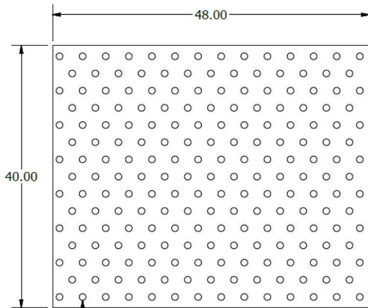
\varnothing 1.00 Embossed Tread TYP 4040 Platform Filler Plate
