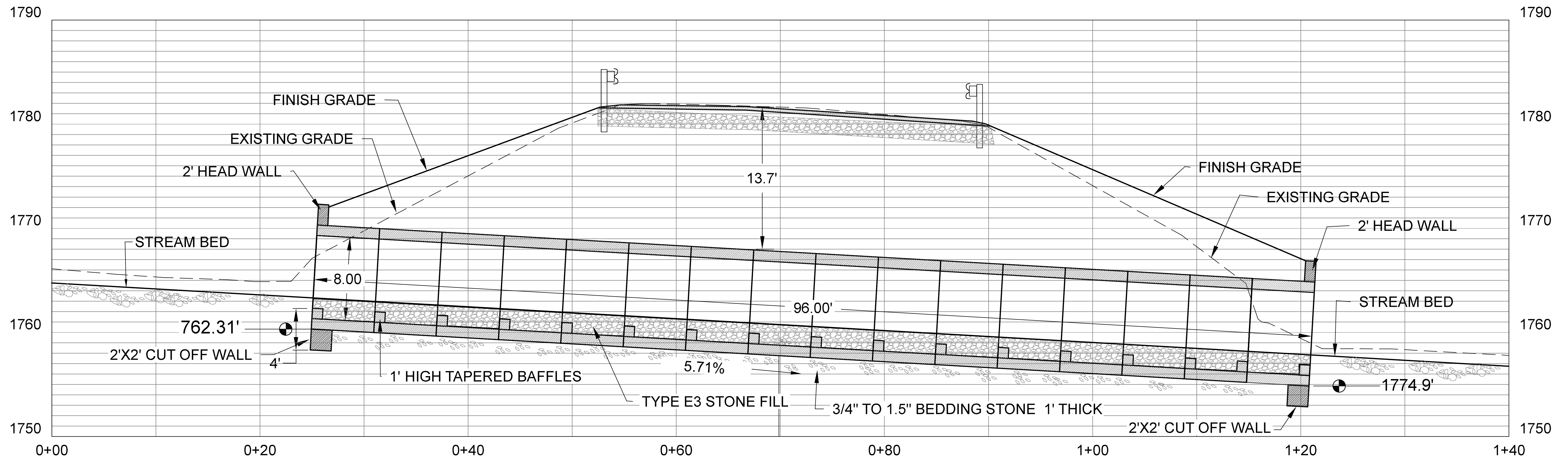
STREAM PROFILE 1"=5' HORZ.; 1"=5' VERT.
