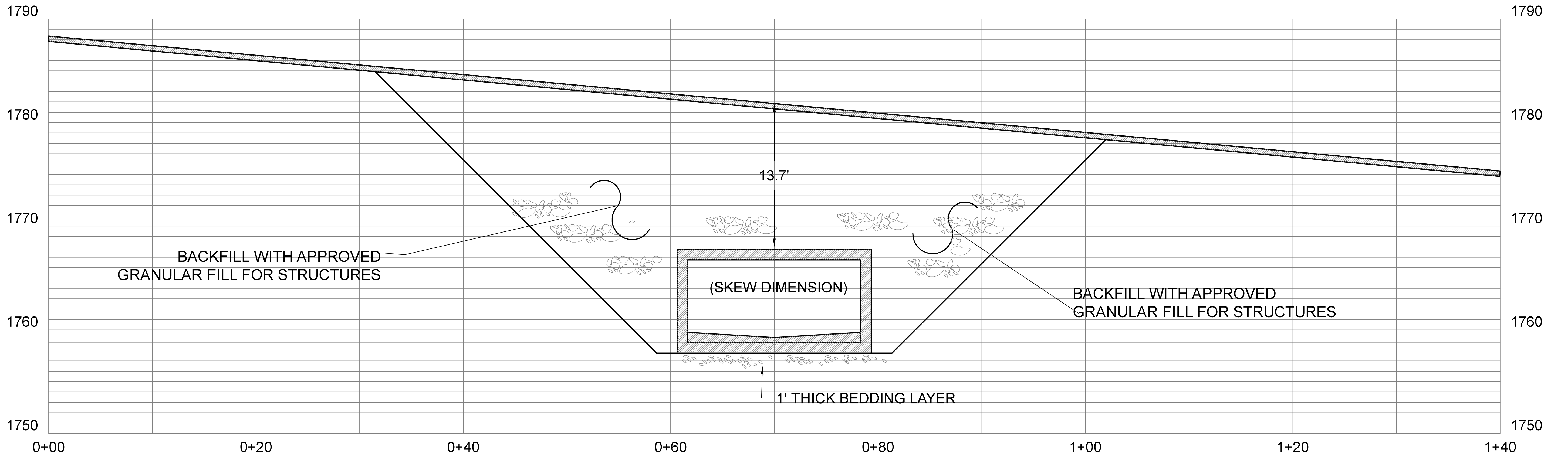
ROAD PROFILE 1"=5' HORZ.; 1"=5' VERT.
