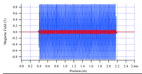
Raw Hall Probe Data
