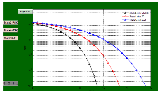
Fig. 3. The relation of symbol error rate (SER) and SNR gain with 4- state PSK and conditions taken for decoding are MMSE and ZF and reduction of noise in transmission state
