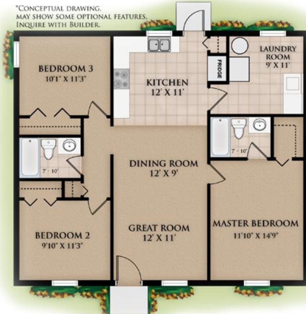
DEVONPORT BUNGALOW 1132 SF LIVING 8' FLAT CEILINGS
