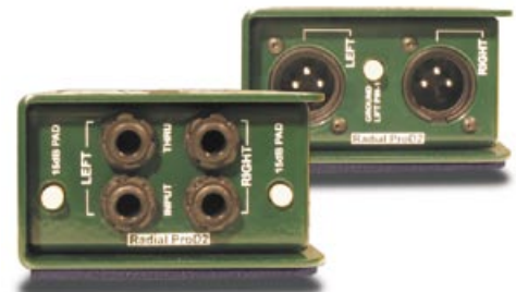
The ProD2 is two independent direct boxes in one: two inputs, thru-puts, pads, transformers, and outputs.
