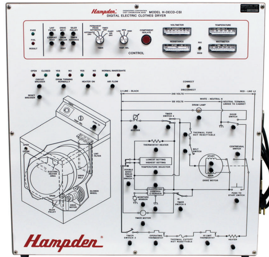
Hampden Model H-DECD-CSI Digital Electric Clothes Dryer Simulator
