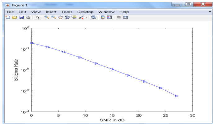
Fig.2: BER and SNR channel error reduction.
