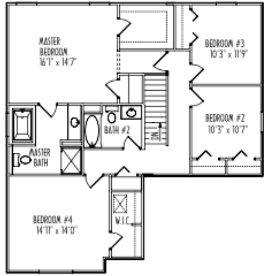
SECOND FLOOR 4 BED
