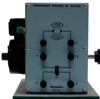
MODEL PM-100 Permanent Magnet DC Motor 1750 rpm 125V 1/3hp
