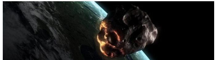
Apophis Asteroid (year 2029-2036)
