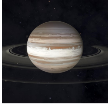
Rings of Jupiter
