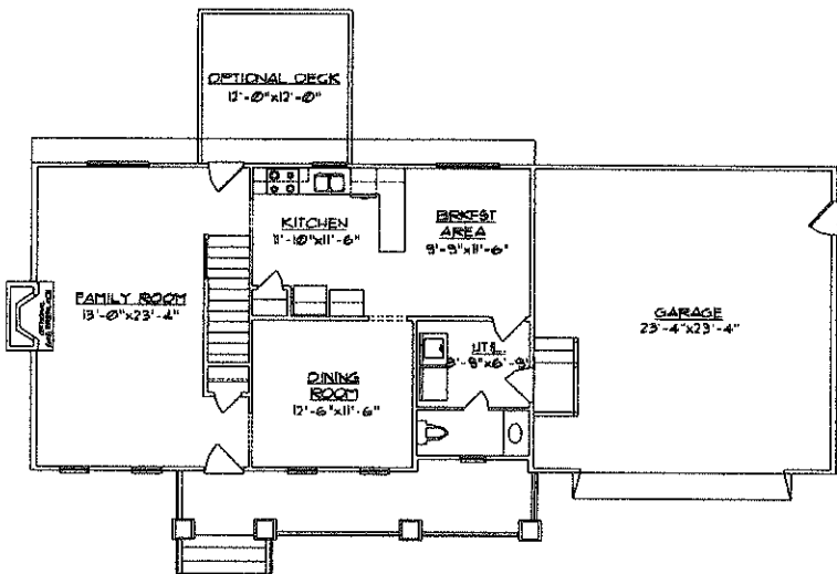
FIRST FLOOR PLAN 927 SQ. FT. (HEATED) 568 SQ. FT. (GARAGE)
