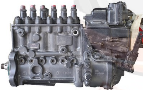
Bosch P7100 Dodge 5.9L
