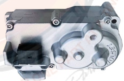
Cummins Electronic VGT Turbocharger Actuator Core
