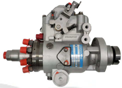
Ford 6.9L
