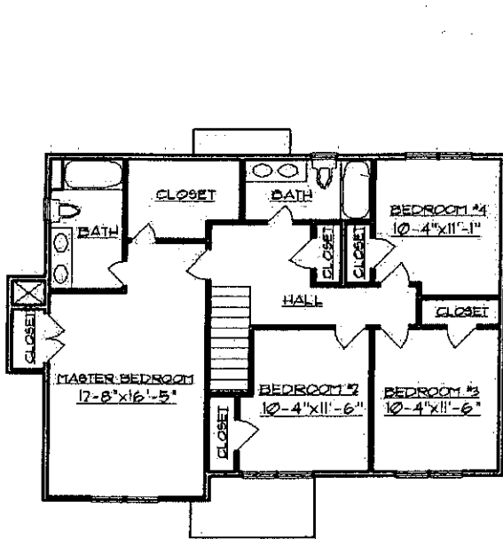
SECOND FLOOR PLAN 1012 SQ. FT. (HEATED)
