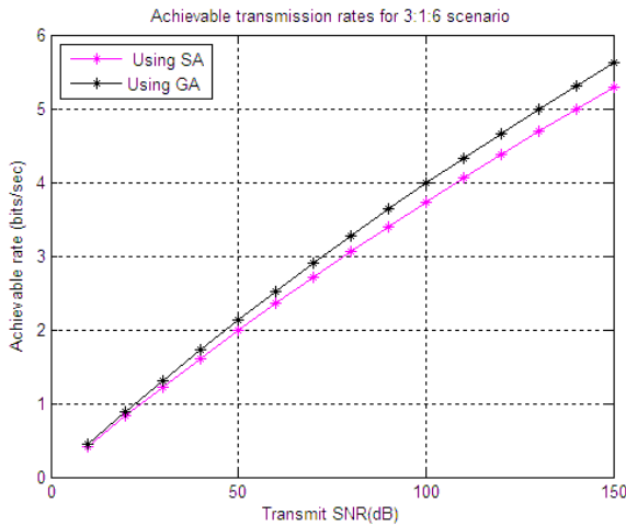
Fig 3: comparison between GA and SA without using MIMO Here in the above graph we transmit the signals showing the coordinates among the ratio test of 3:1:6 scenarios for presence of achievable transmission among the antenna by using genetic algorithm and simulated annealing process by that we can generate the signal much efficient
