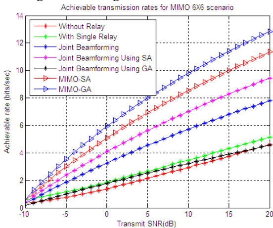
Fig4: Comparison of achievable transmission of SNR Here in the above graph the signal propagated by the comparison among the approx bits of 6X6 scenario by all generated transmission rates here we can show the efficient of 90% signal by using MIMO-GA and MIMO-SA and there is no complexity among the signals
