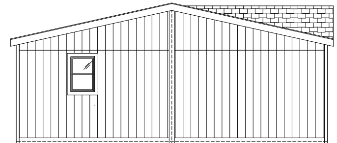
REAR ENDWALL
