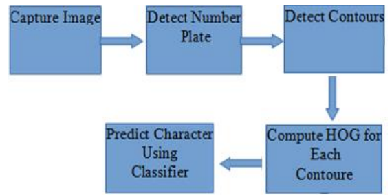
Fig.2: Testing Procedure of Custom Neural Network
