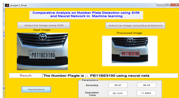
Fig.14: GUI with results after detection using neural network.
