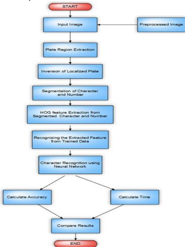
Fig.5: Flowchart of Proposed Method
