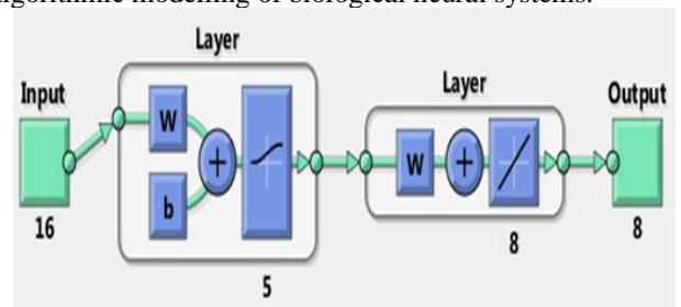
Fig.4: Custom Neural Network of Proposed Method
