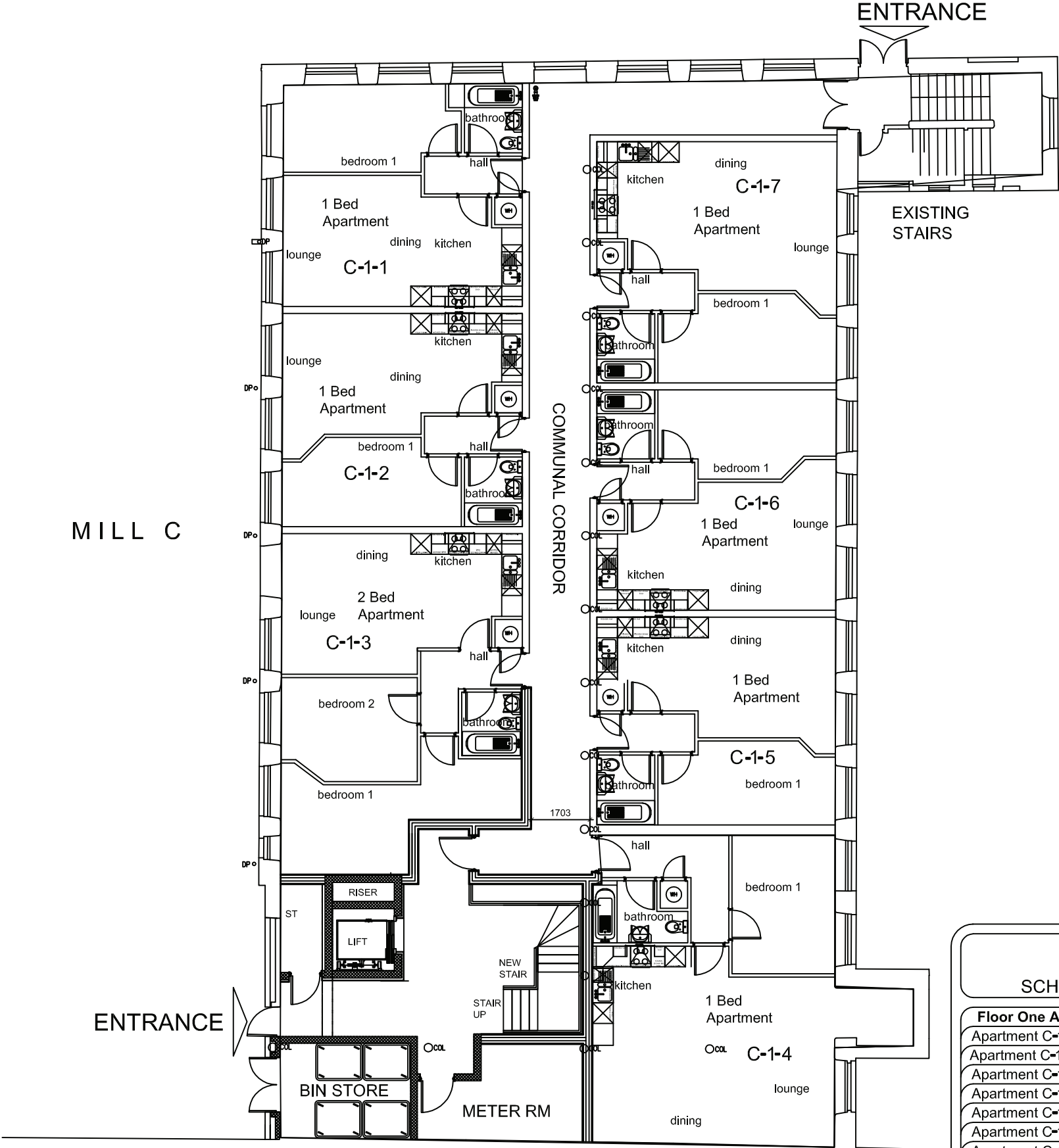
PROPOSED FLOOR ONE PLAN
