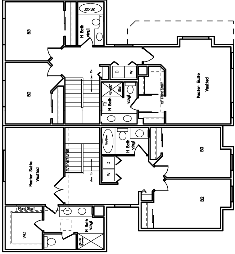
Tulip Master Rear SECOND FLOOR Tulip Master Front
