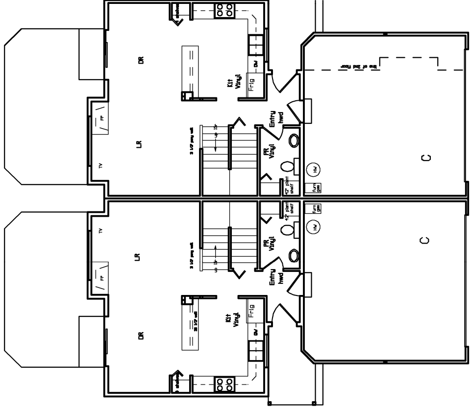
Tulip Master Rear FIRST FLOOR Tulip Master Front
