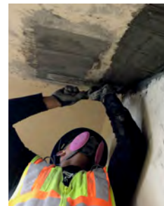
Soffit repair
