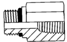
FEMALE PIPE ADAPTER 0502 (F5OG-S)
