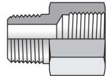
Conversion Adapter NPT-BSPP (FHG4)
