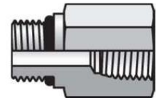
Conversion Adapter SAE-ORB / BSPP (F5OHG4)
