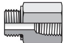
Conversion Adapter METRIC-ORR (F8OHG)
