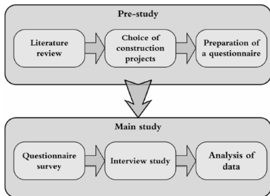
Figure 1. Research Design.
