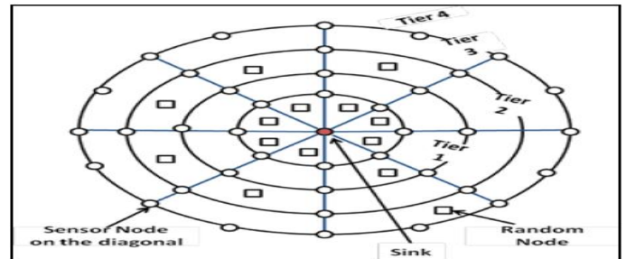
[, Fig.7] Circular Topology
