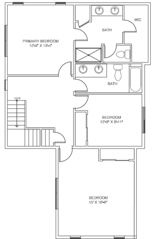
3RD FLOOR
