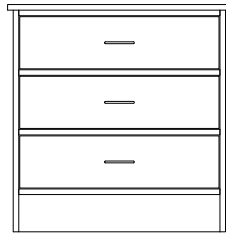
3 Drawer Chest 30" W, 20" D, 30" H (BAY-400)
