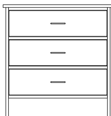
3 Drawer Chest 30" W, 20" D, 30" H (CEN-400)
