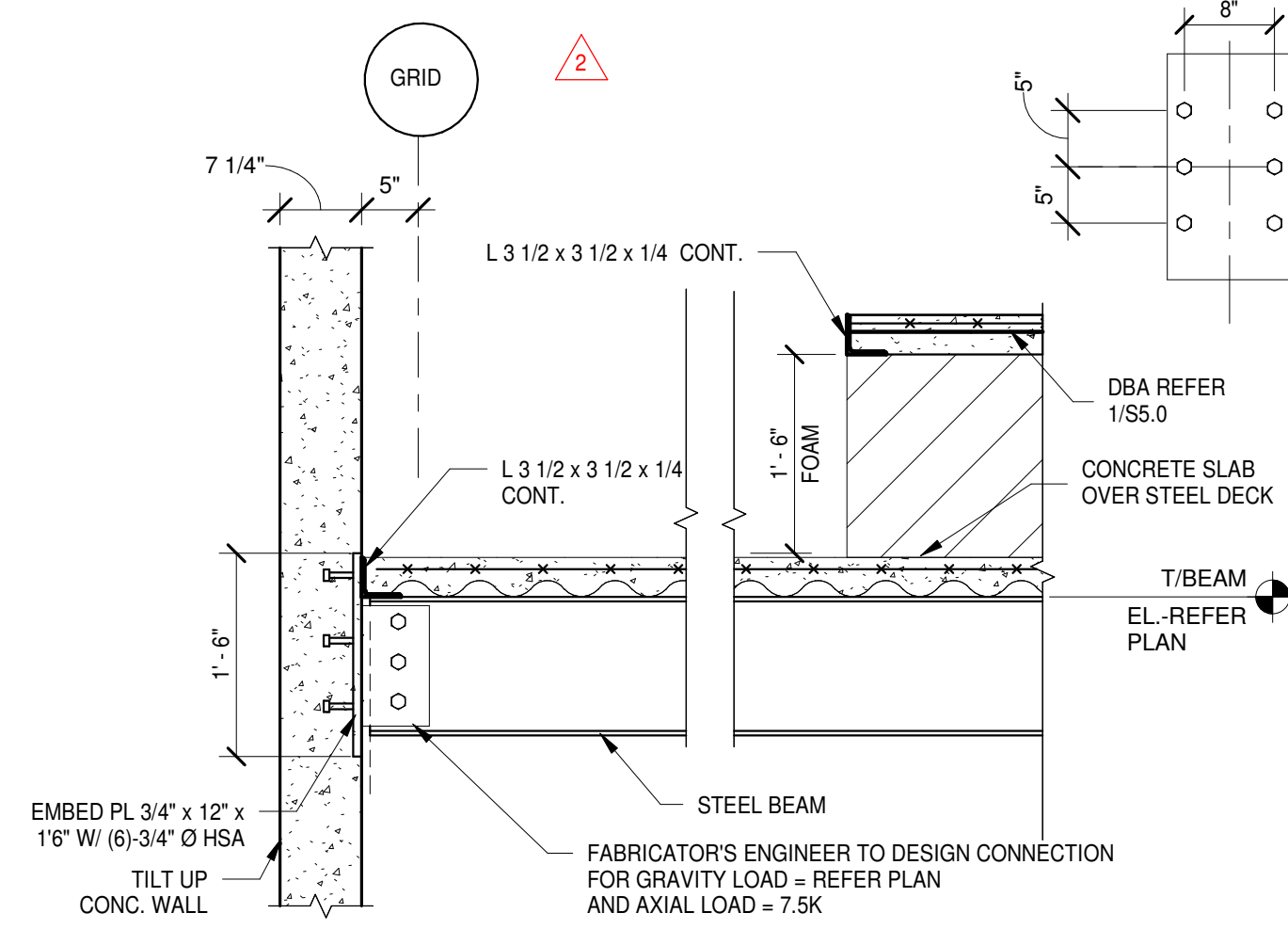
BEAM BEARING SECTION AT 2ND FLOOR
