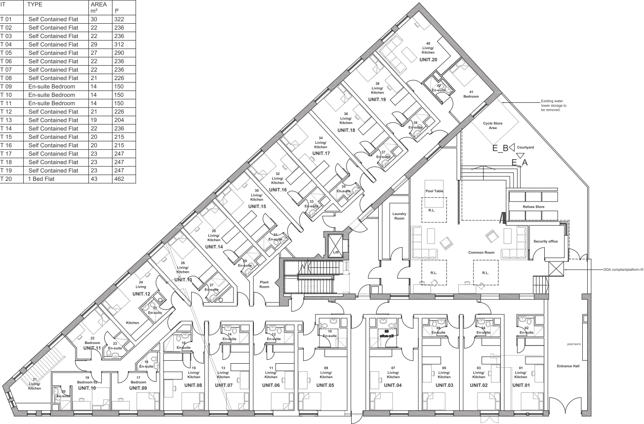
GROUND FLOOR FLAT UNIT AREA SCHEDULE
