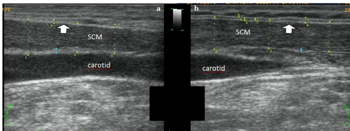
Fig. 2 a SCM in control subject (arrow fascia). b SCM in a patient (arrow fascia)
