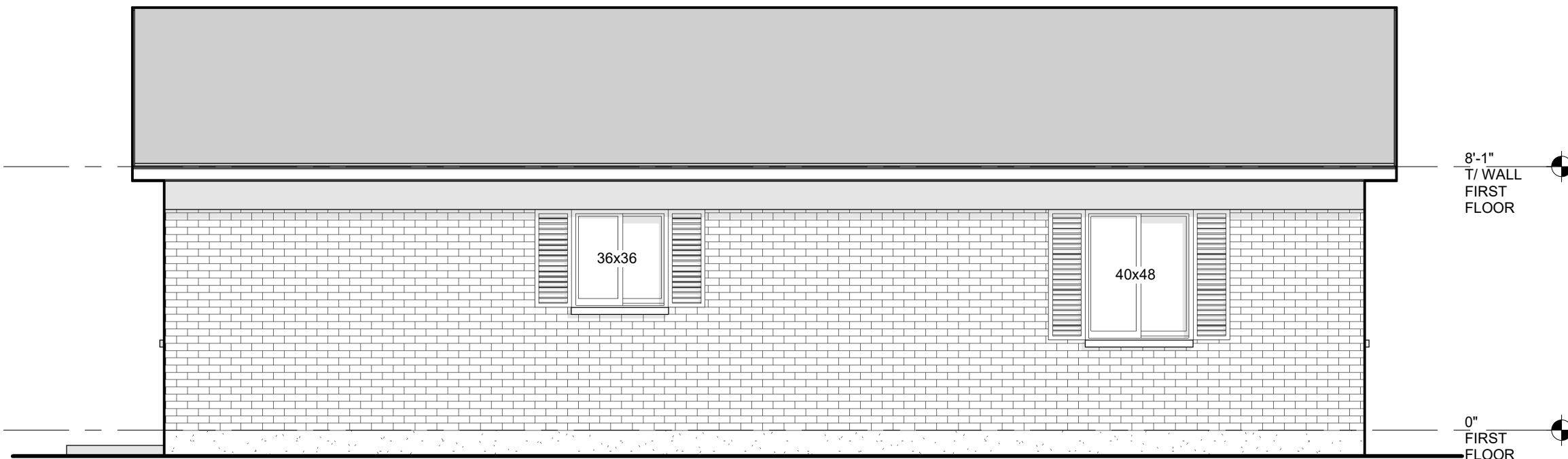
BUILDING TYPE E REAR ELEVATION
