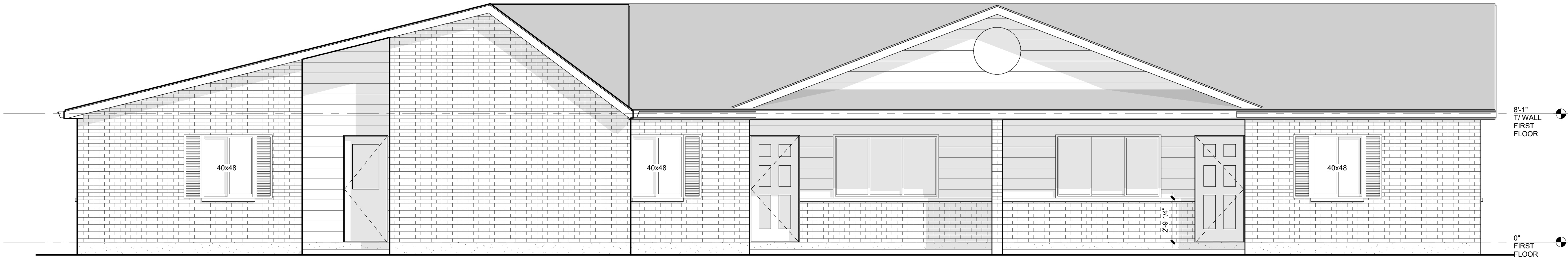
BUILDING TYPE C FRONT ELEVATION
