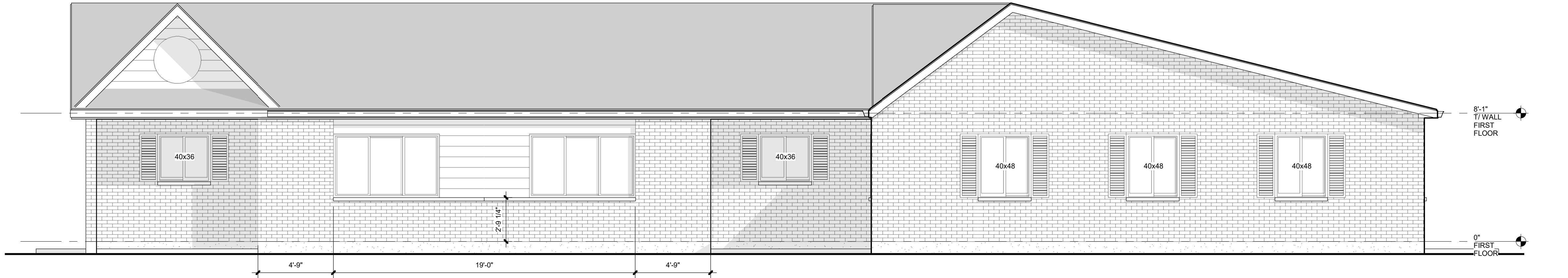
BUILDING TYPE C RIGHT ELEVATION
