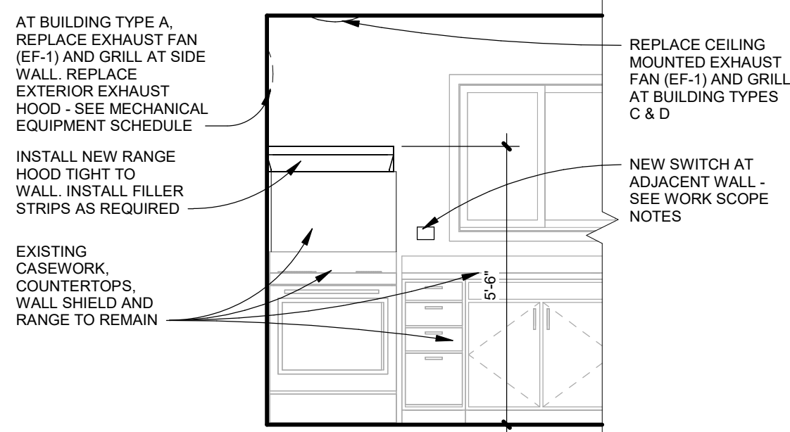
2-BEDROOM KITCHEN ELEVATION
