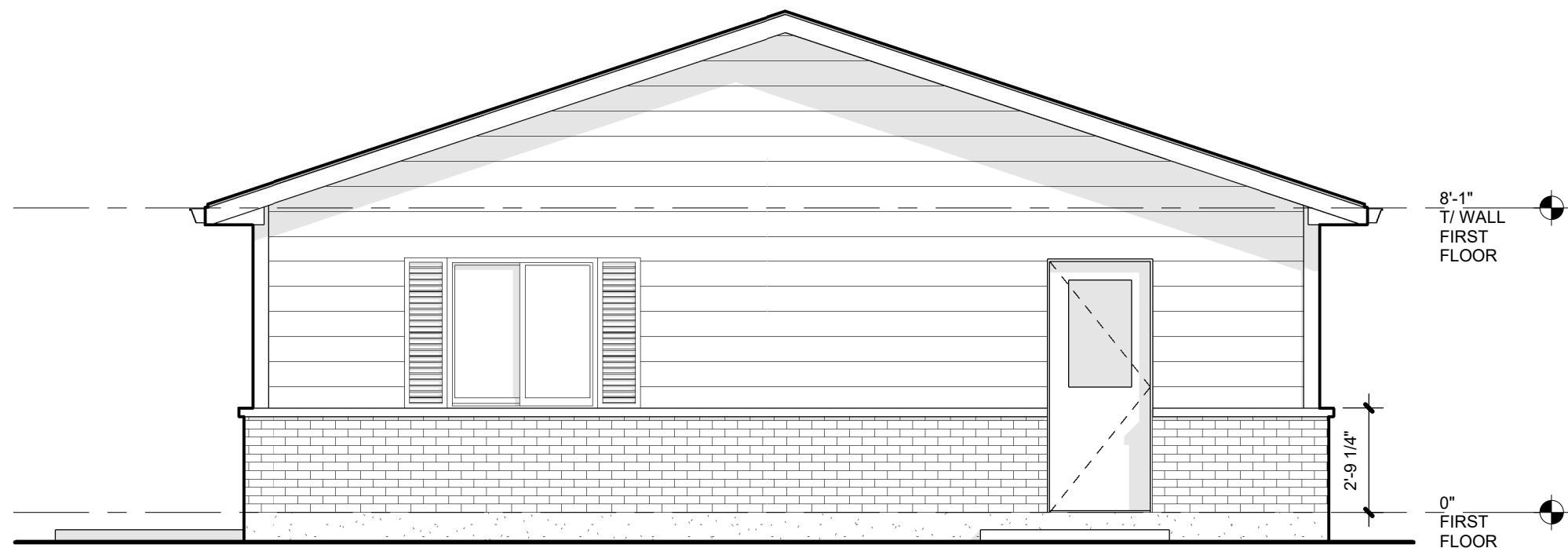
BUILDING TYPE F RIGHT ELEVATION
