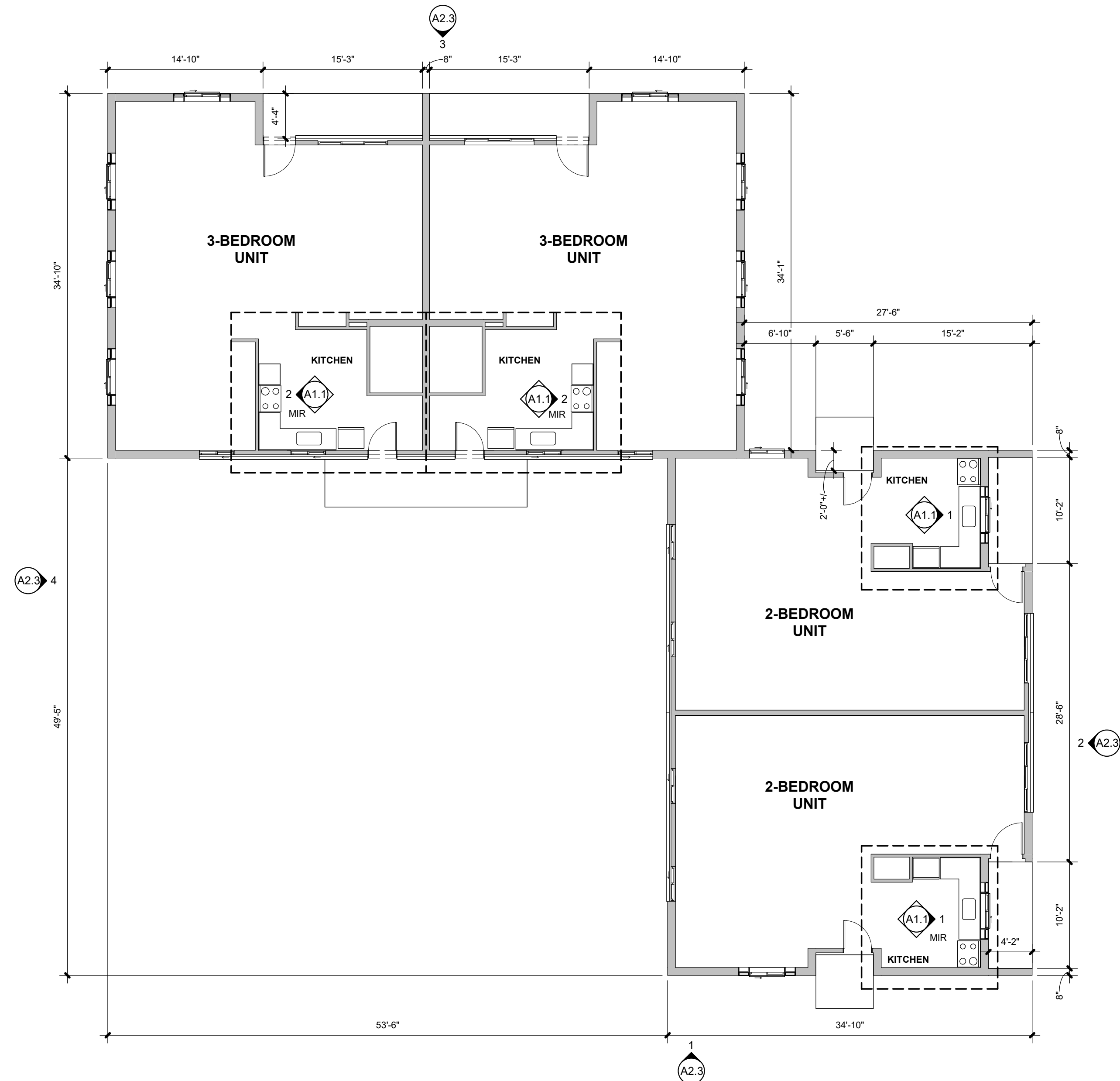
BUILDING TYPE D SCALE: 1/8" = 1'-0"
