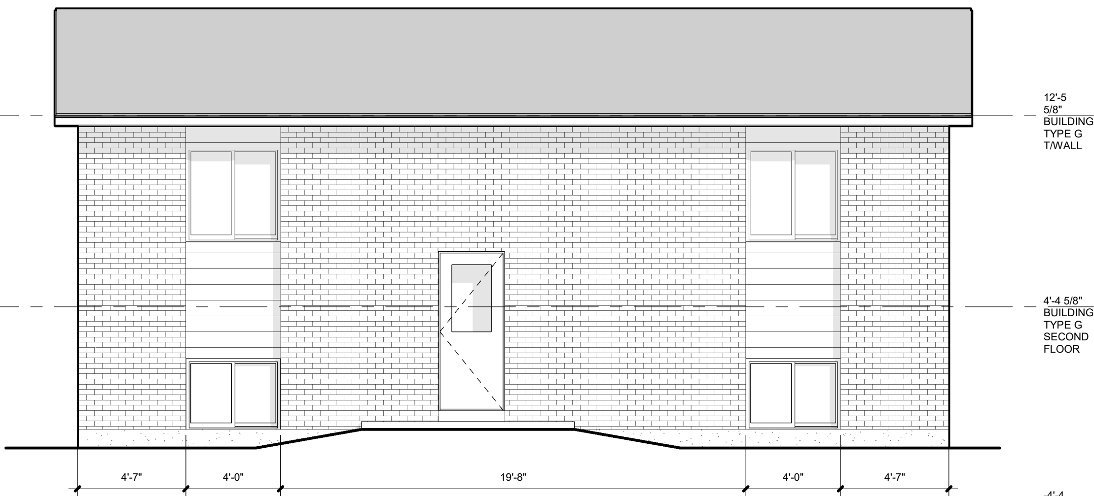
BUILDING TYPE G REAR ELEVATION
