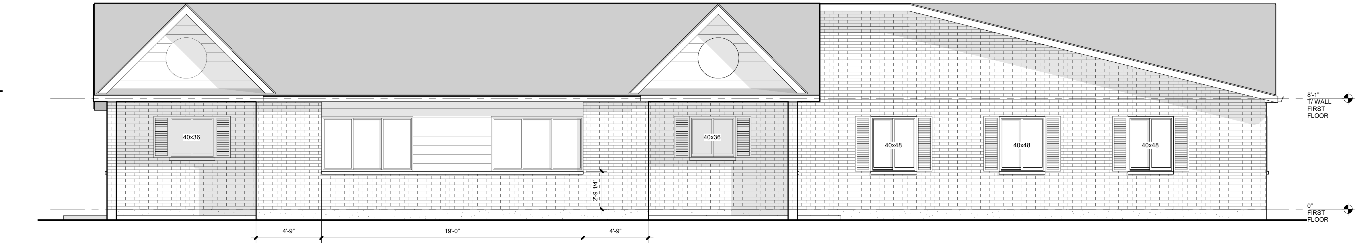
BUILDING TYPE D RIGHT ELEVATION
