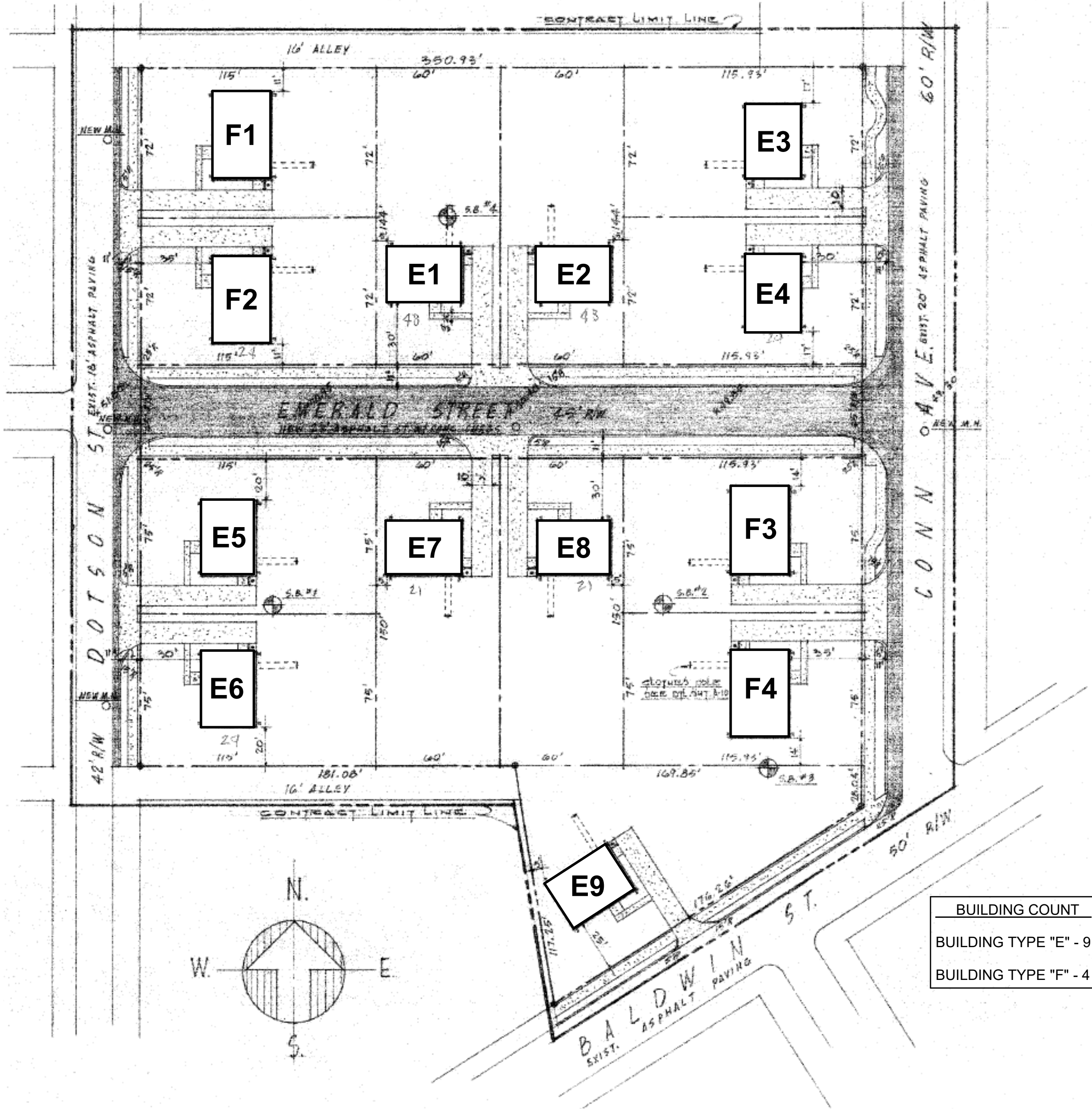
SITE PLAN A
