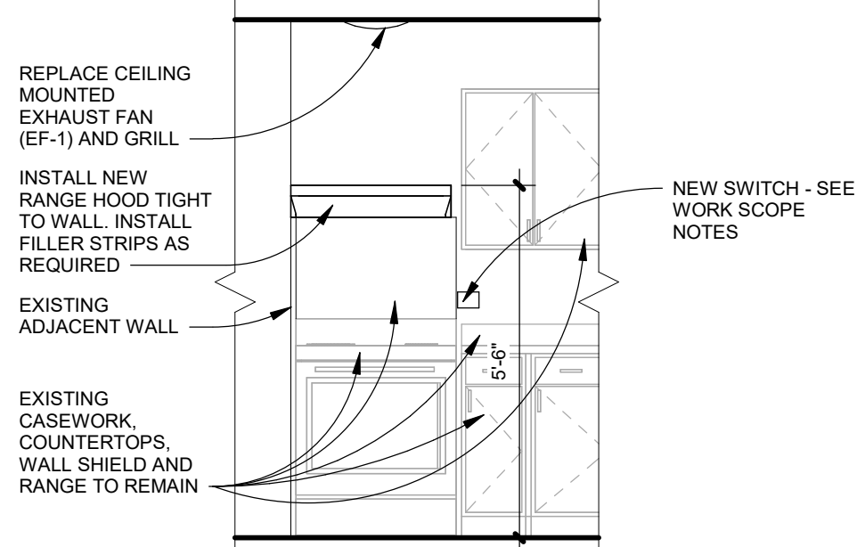
3 & 4 BEDROOM HOUSE KITCHEN ELEVATION
