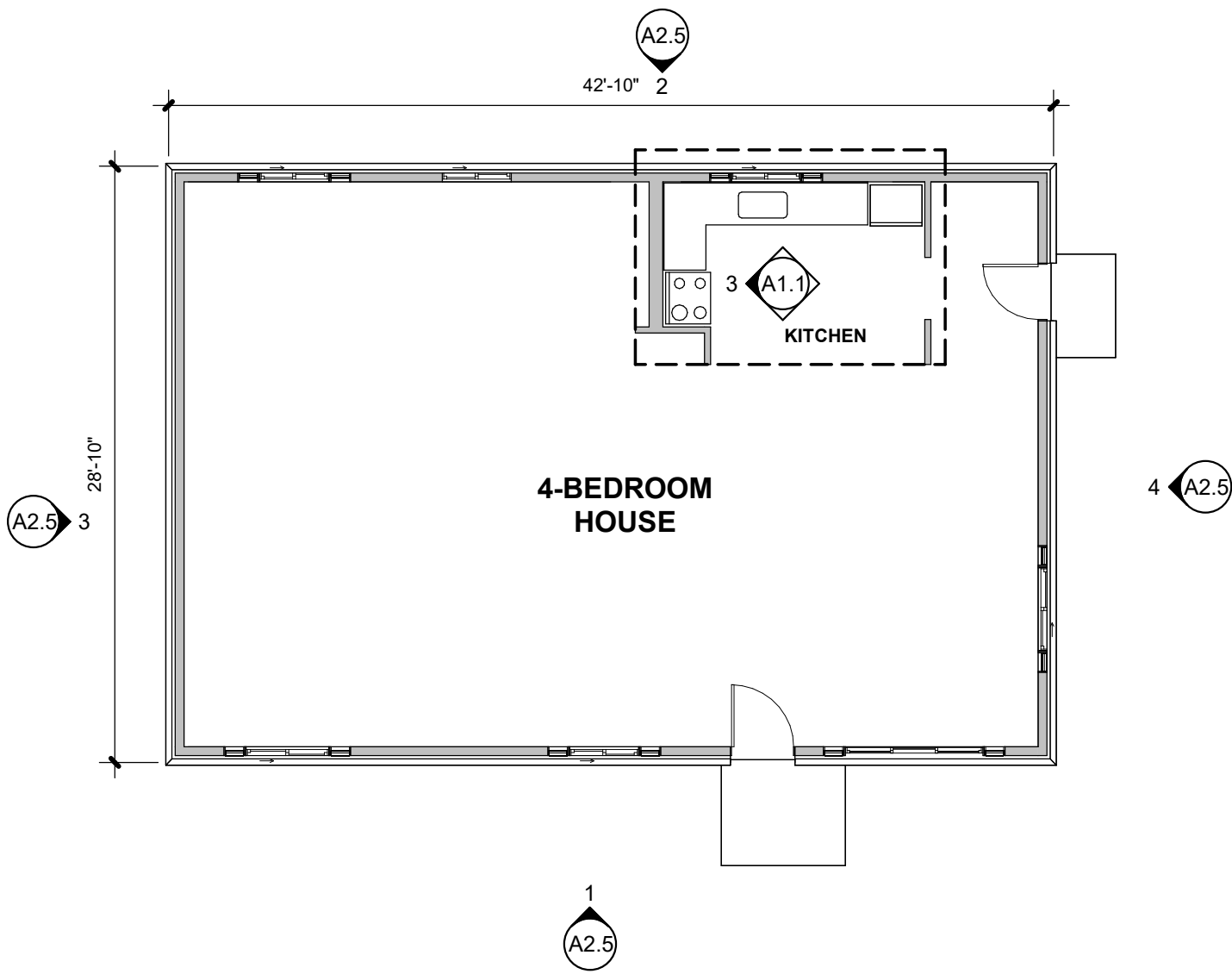
BUILDING TYPE F
