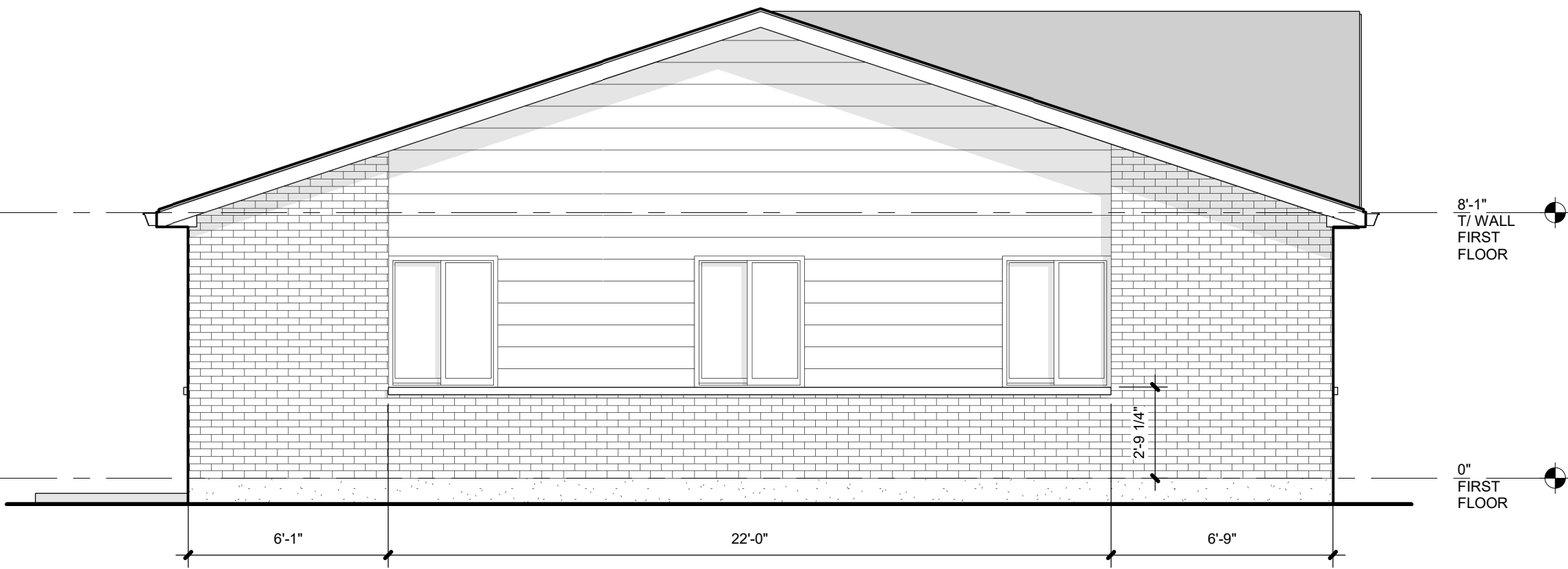
BUILDING TYPE B LEFT ELEVATION
