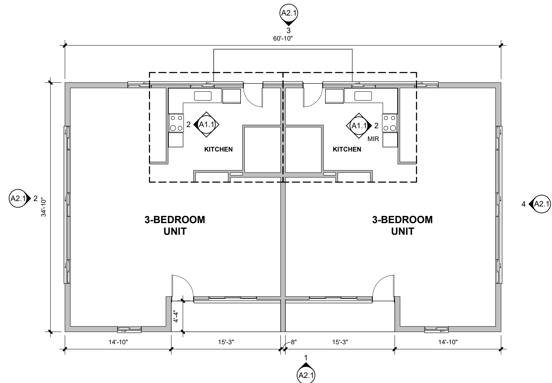
BUILDING TYPE B SCALE: 1/8" = 1'-0"
