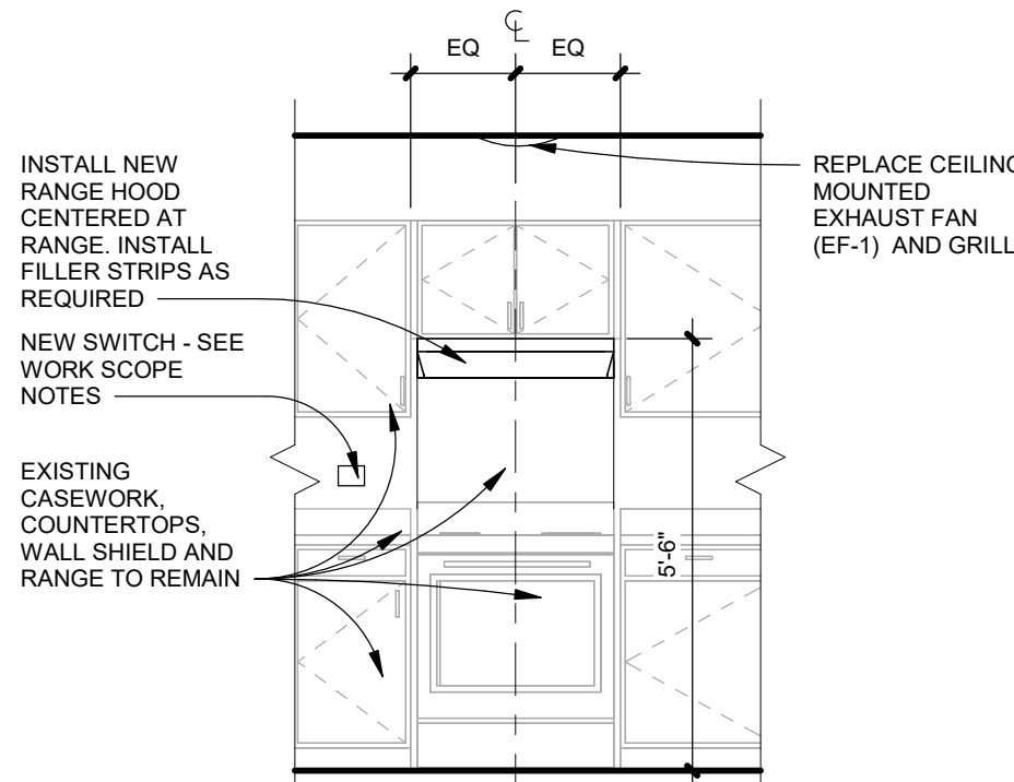
3-BEDROOM KITCHEN ELEVATION
