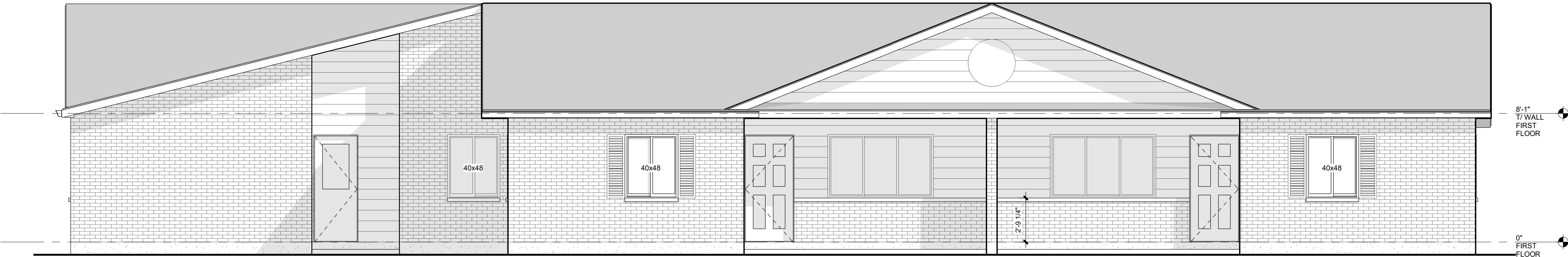
BUILDING TYPE D REAR ELEVATION
