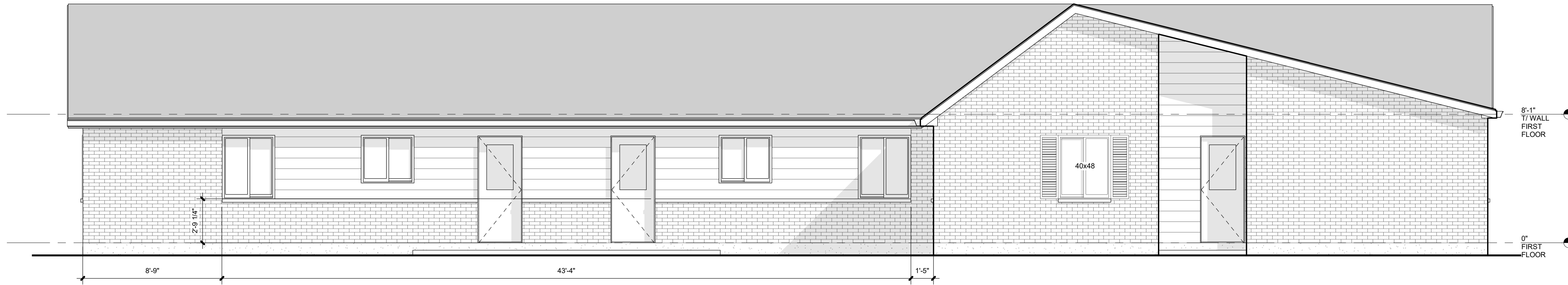
BUILDING TYPE D FRONT ELEVATION
