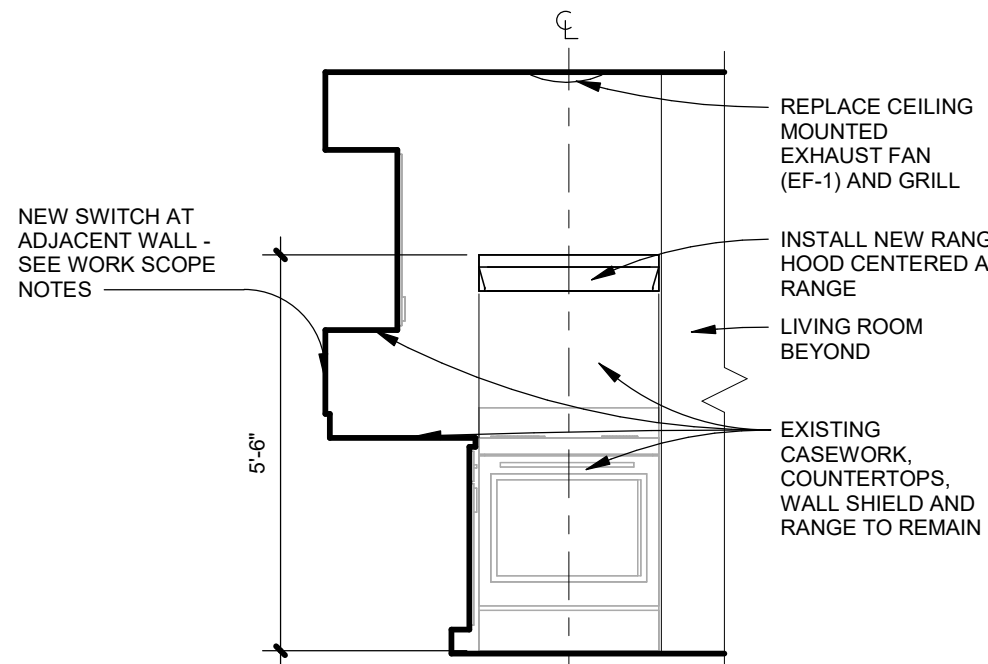
5 BEDROOM HOUSE KITCHEN ELEVATION
