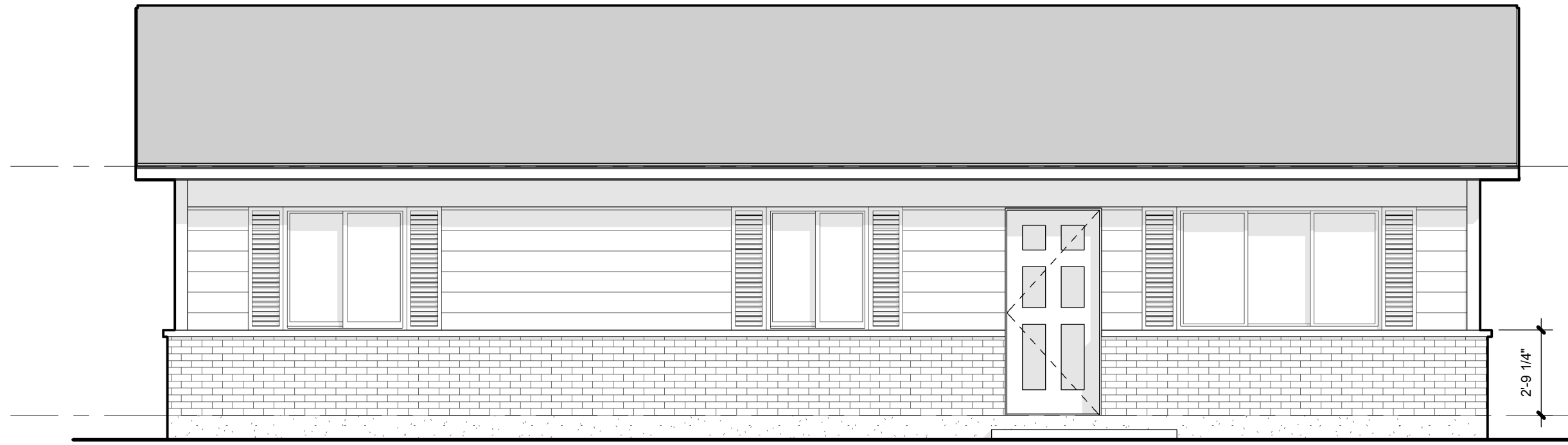
BUILDING TYPE F FRONT ELEVATION
