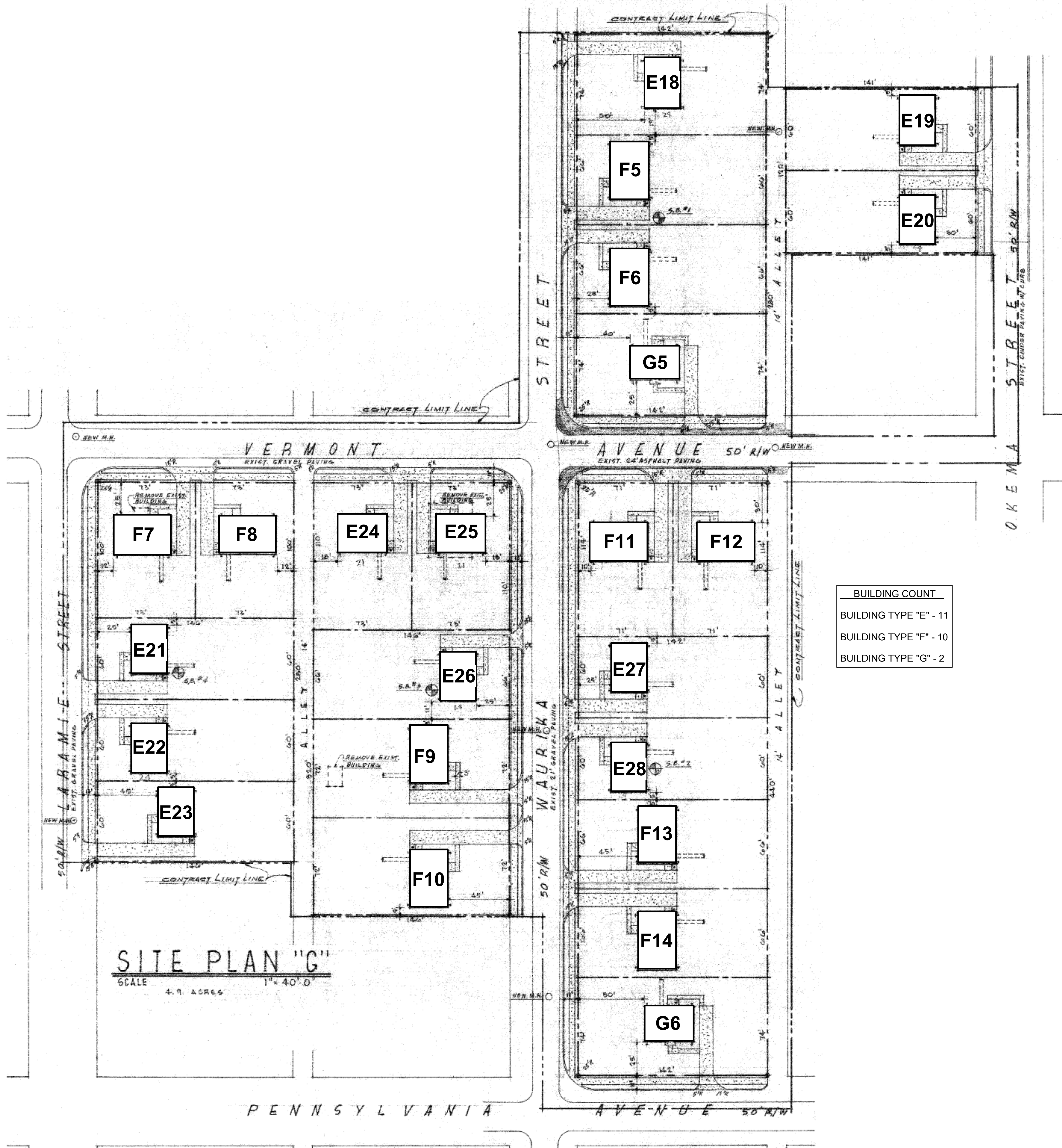
SITE PLAN G SCALE: 1" = 40'-0"
