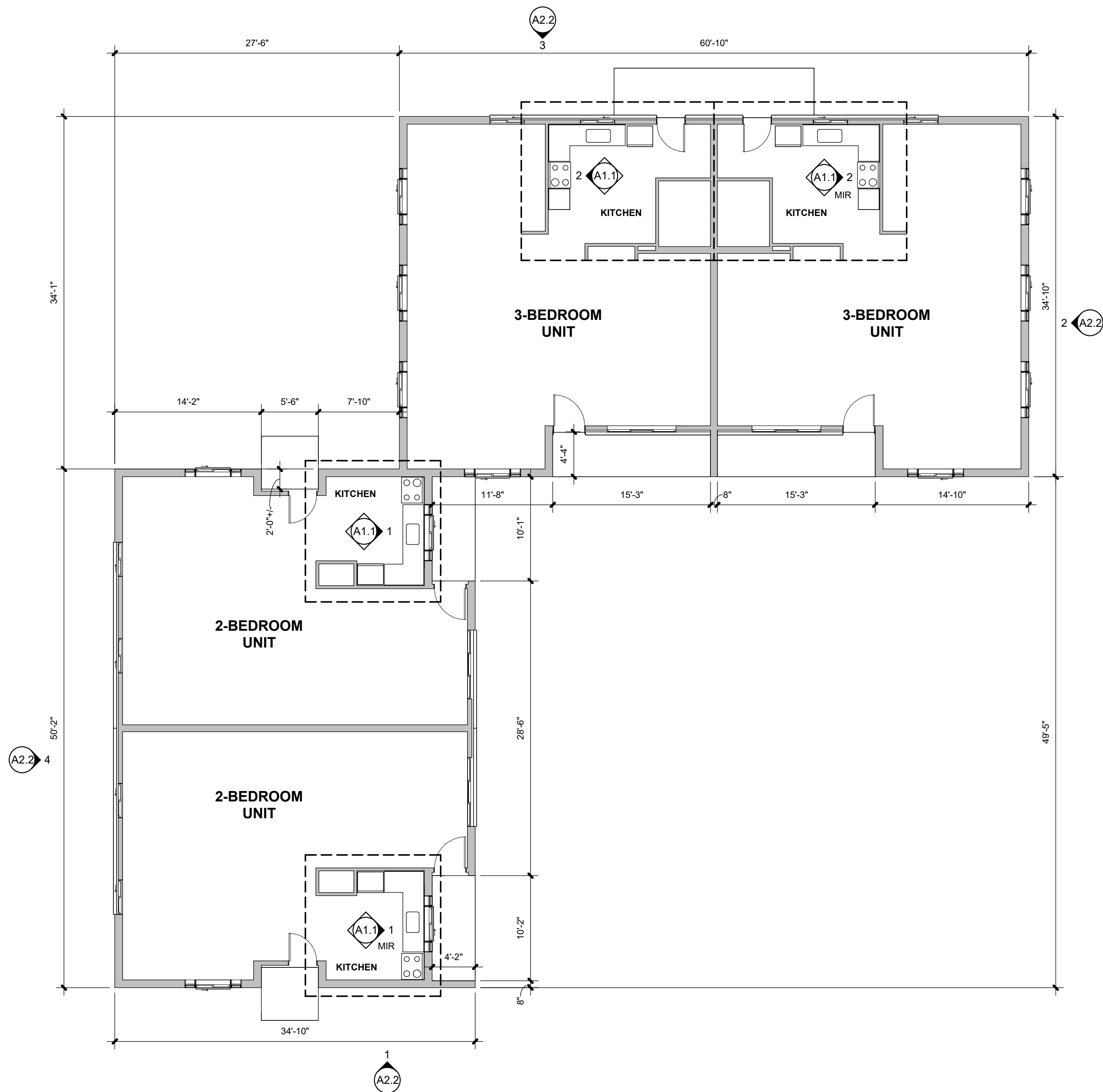
BUILDING TYPE C SCALE: 1/8" = 1'-0"
