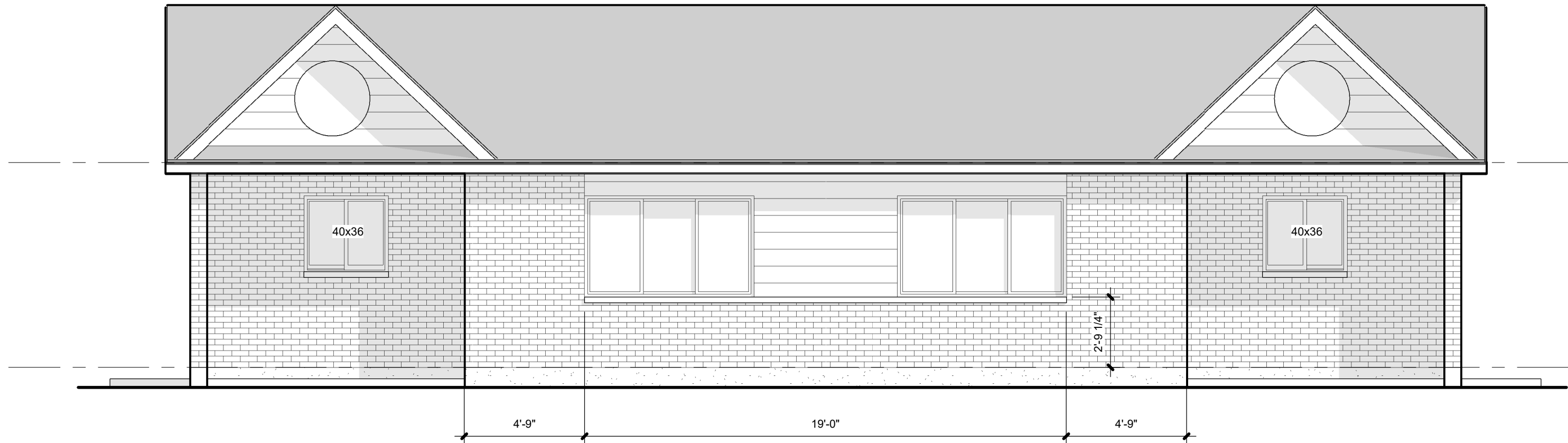
BUILDING TYPE A FRONT ELEVATION
