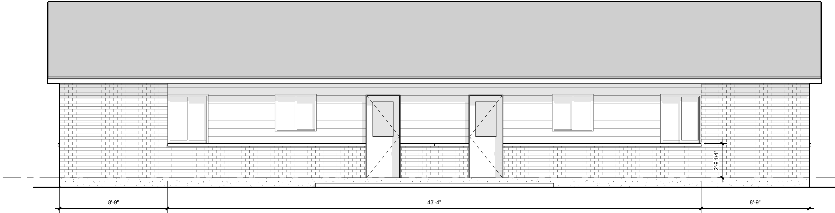
BUILDING TYPE B REAR ELEVATION
