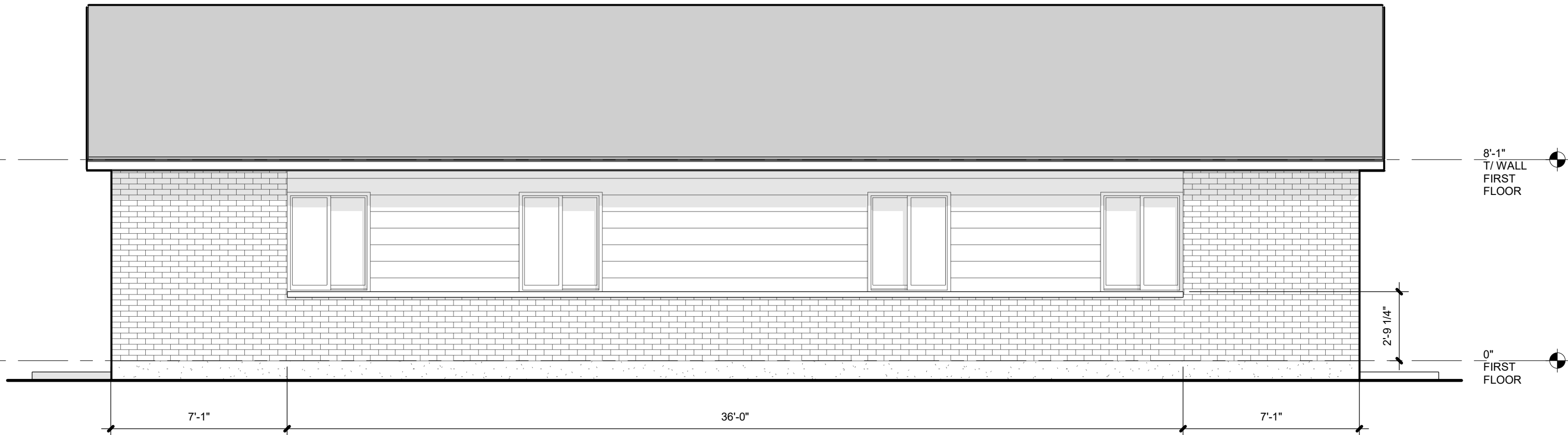
BUILDING TYPE A REAR ELEVATION
