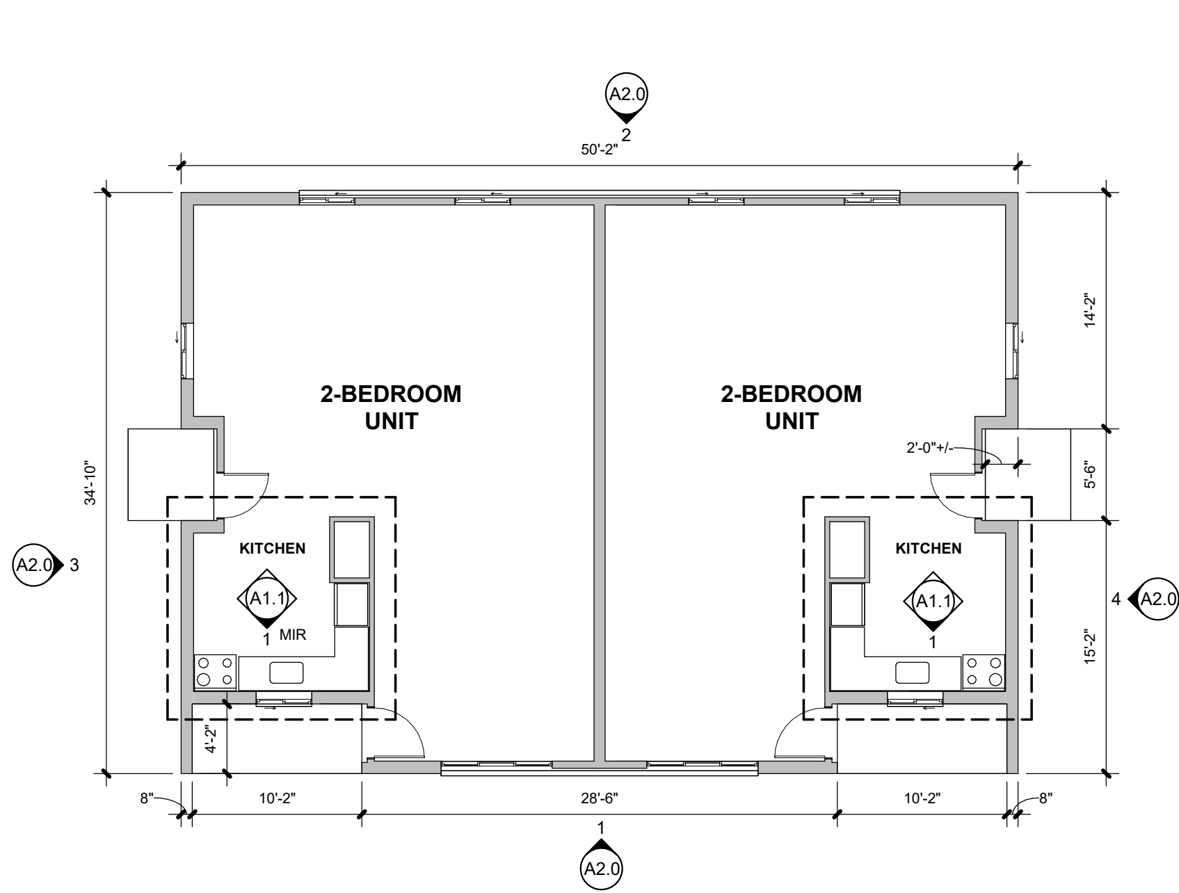
BUILDING TYPE A SCALE: 1/8" = 1'-0"
