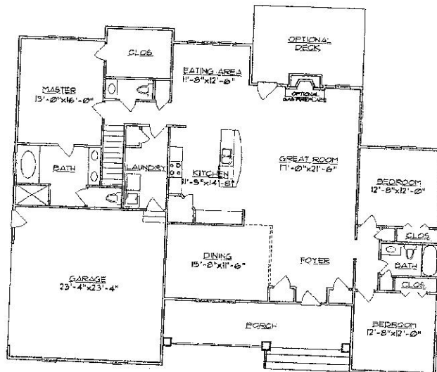
FIRST FLOOR PLAN 2152 SQ. FT. (HEATED) 564 SQ. FT. (GARAGE)
